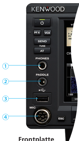
Frontplatte
